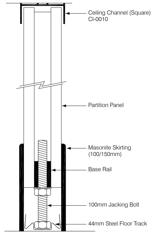
Full Height 'H' Type Elevation
