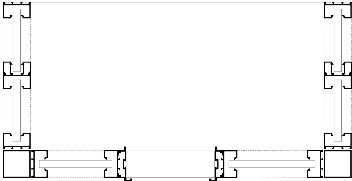
DOOR JAMB DETAIL WITH 26MM FRAME
