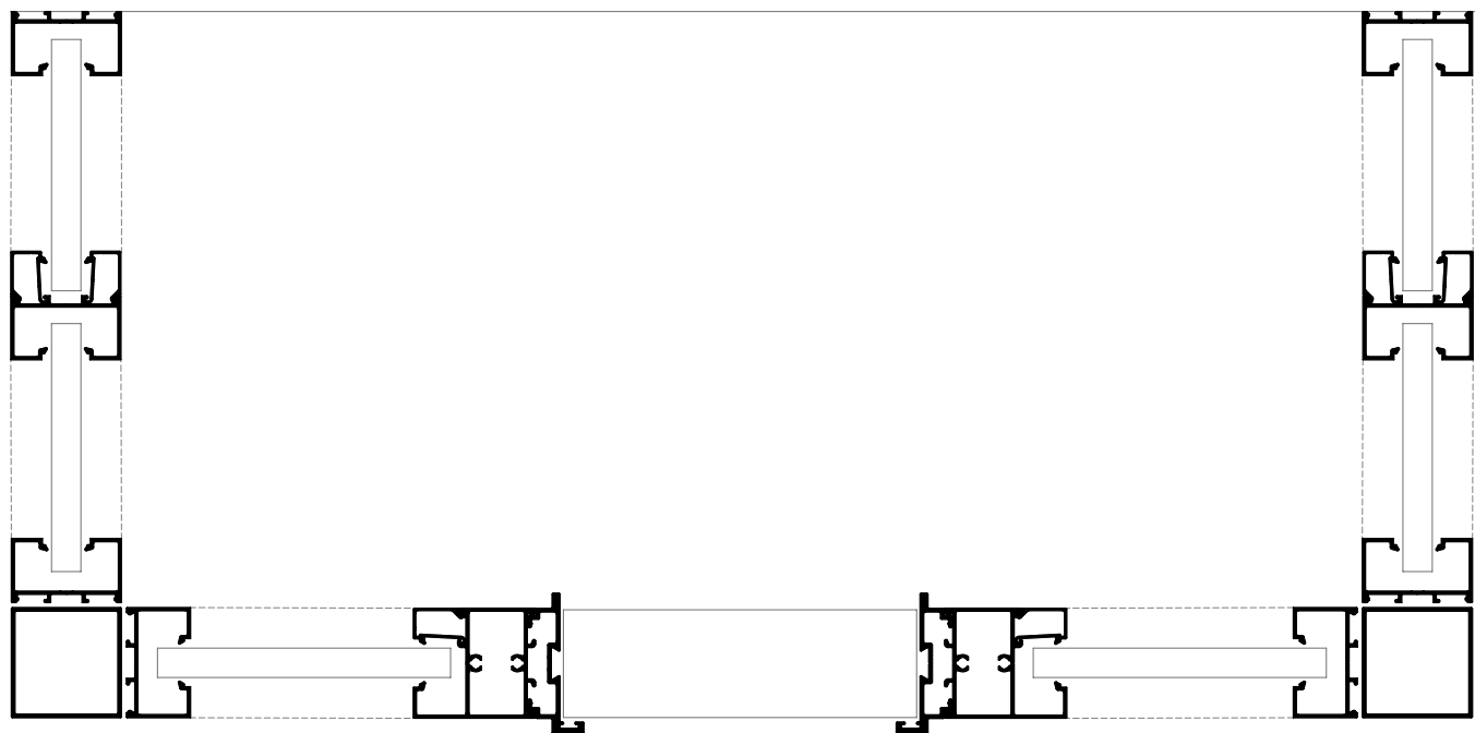
DOOR JAMB DETAIL WITH 50MM FRAME
